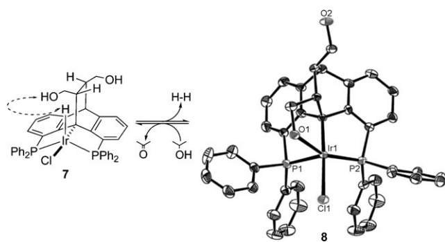
Scheme 1. ORTEP drawing with the ellipsoids shown at 50% probability. Hydrogen atoms and solvent molecules are omitted for clarity. Selected bond lengths [Å] and angles [deg.]: Cl1–Ir1 (2.037(7)), Ir1–P1 (2.365(2)), Ir1–P2 (2.203(2)), Ir1–O1 (2.236(6)); P1–Ir1–Cl1 (97.14(7)), Cl1–Ir1–P1 (84.0(2)), O1–Ir1–P1 (88.58(16)), P2–Ir1–O1 (156.15(16)), P2–Ir1–P1 (109.83(8)), Cl1–Ir1–Cl1 (175.0(2)).
